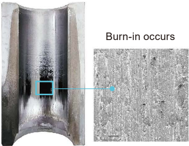
Bonderized Part
